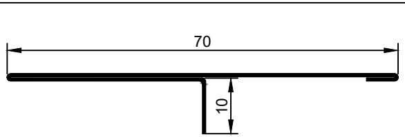
BCR SS T Shape Tile Trim FINISHES: Mirror Length of 2.6 M Ref: TTSST70x10MI
